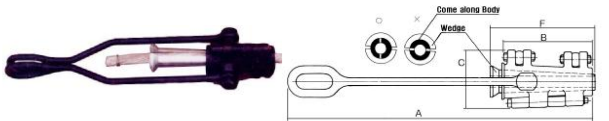
WEDGE TYPE(CW9-W)
