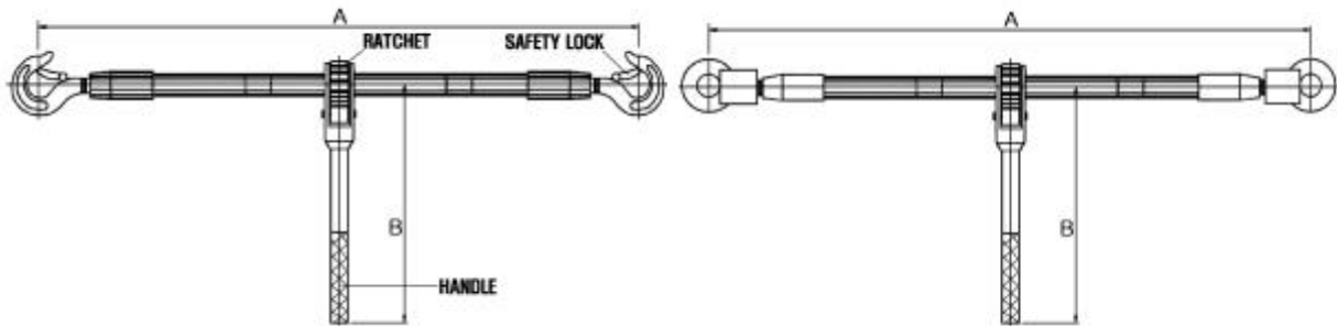
HOOK TYPE
