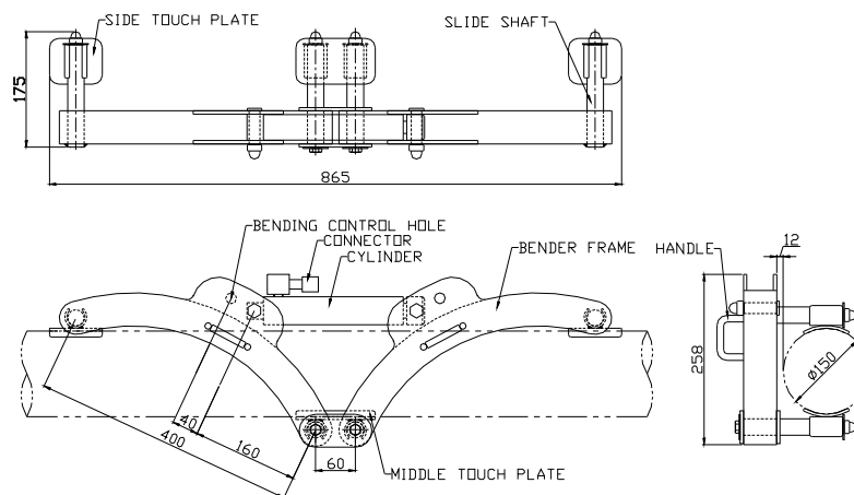
BENDER BODY
